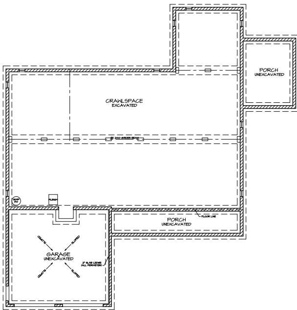
FOUNDATION PLAN A-1 SCALE: 1/4"=1'-0"
