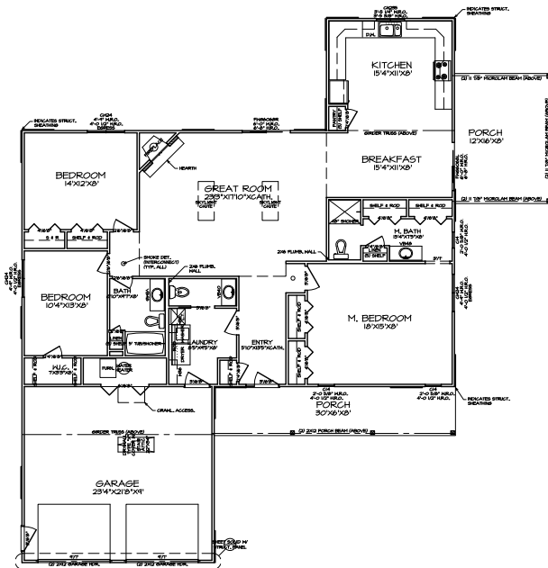
FIRST FLOOR PLAN A-1 SCALE: 1/4"=1'-0"
